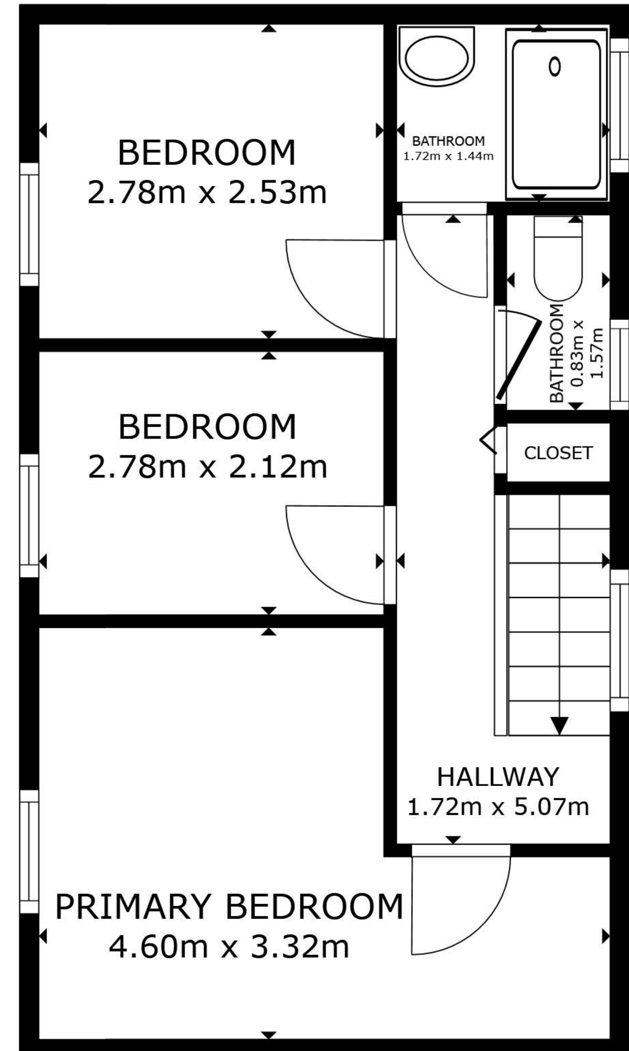
FLOOR 2
