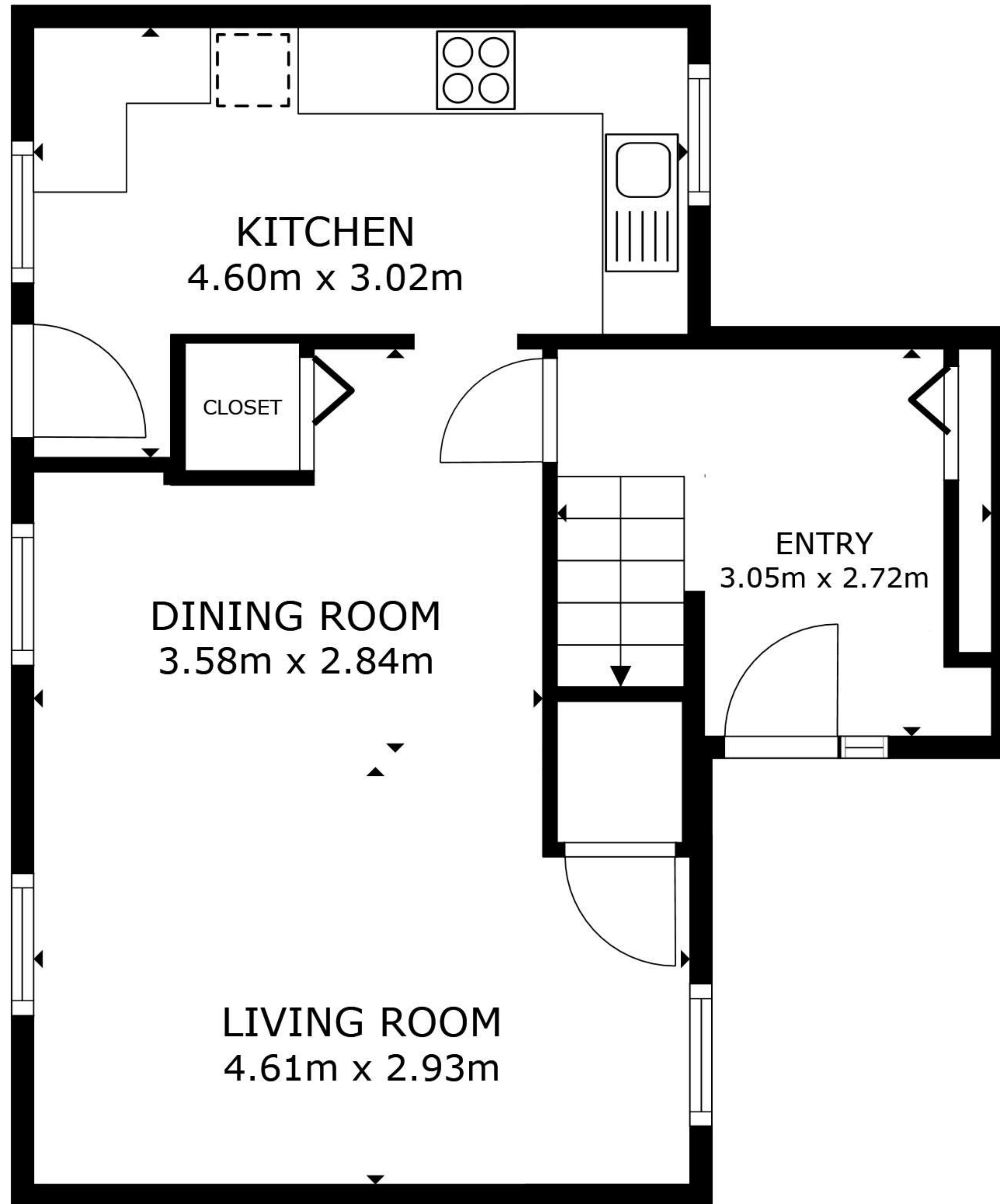
FLOOR 1
