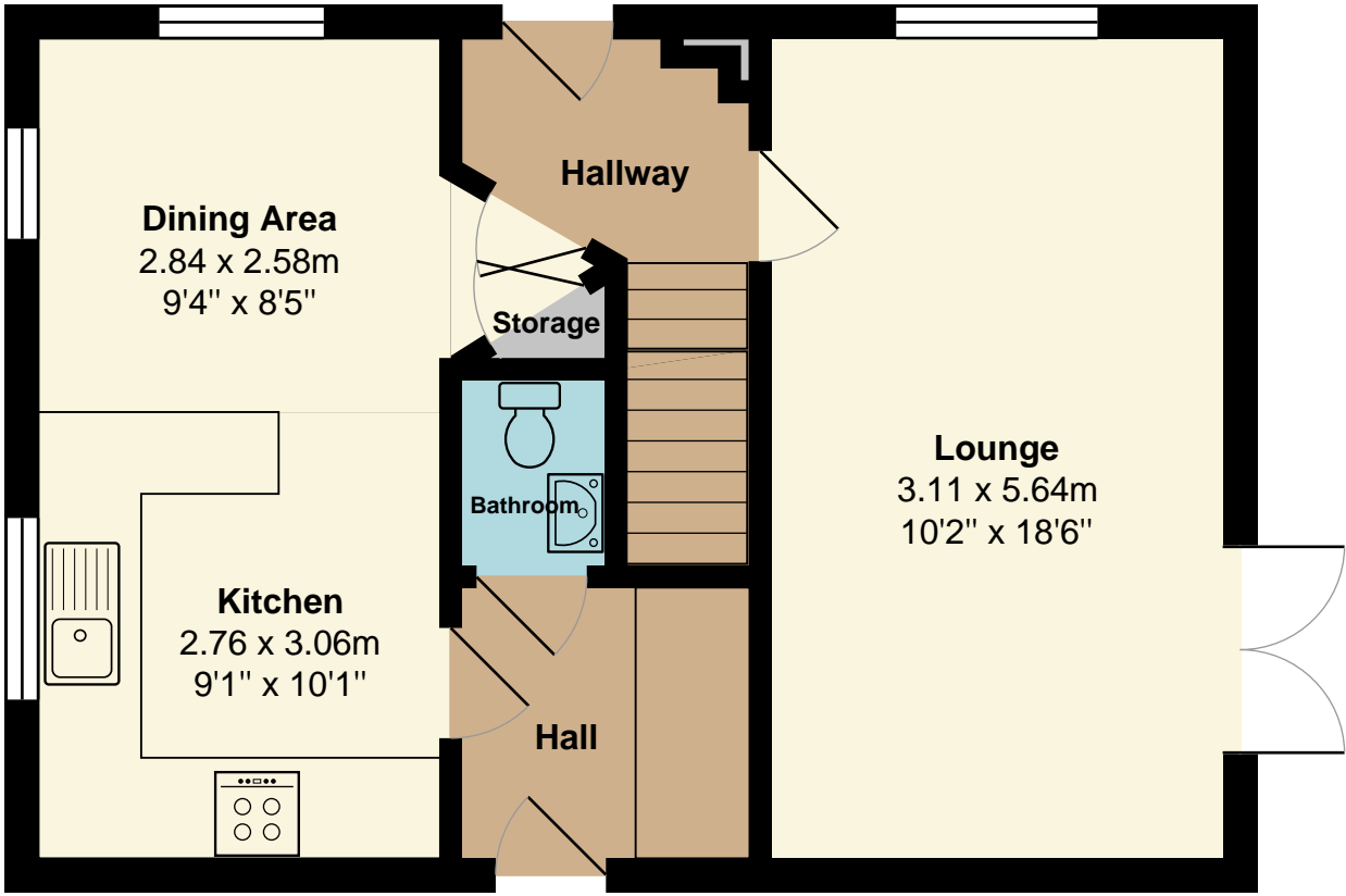
Ground Floor Area: 46.0 m 2 ... 495 ft 2
